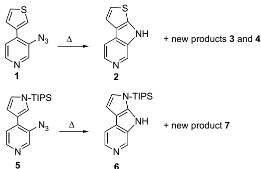
Scheme 1. Cyclisation to \beta -carboline analogues.
