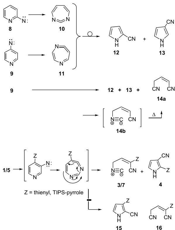
Scheme 5.
